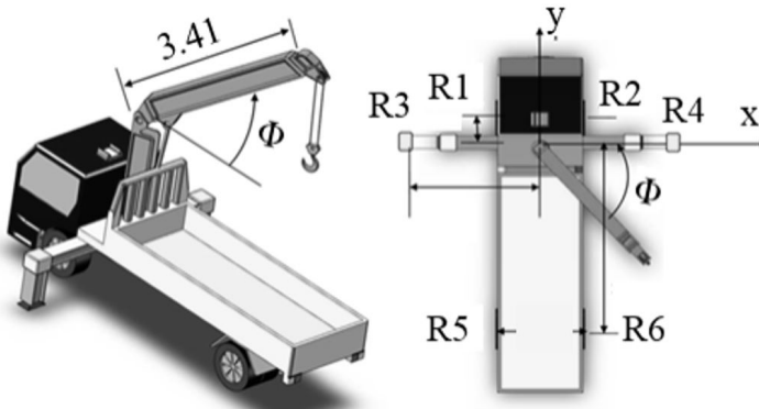
Figure 1: Detailed example for the calculation – Overturning Protection [5].
