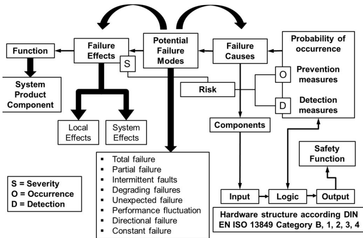
Figure 15: Proposed safety-related solution III, based on AIAG & VDA [6], with modified structure according to ISO 13849 [1] [2].
