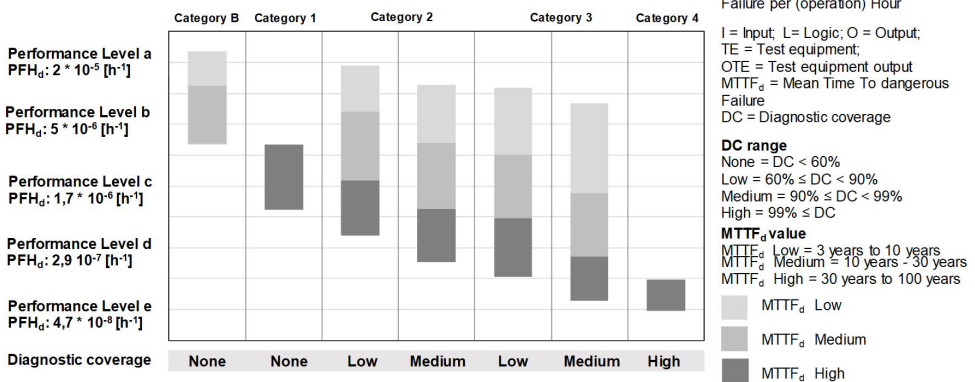
Figure 2: Relationship between categories and PL according ISO 13849 [1] [2].
